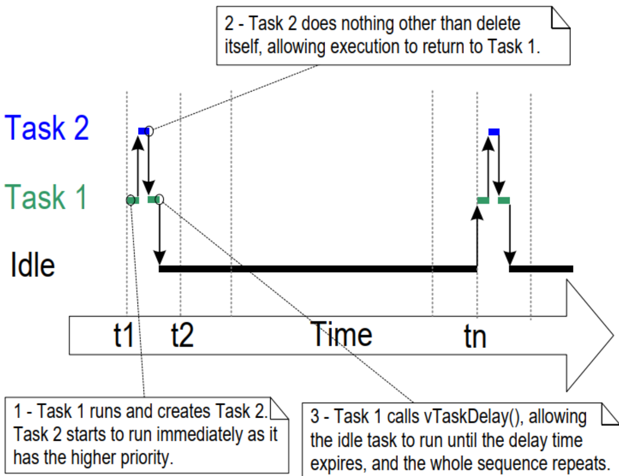
Figure 4.17 The execution sequence for Example 4.9
