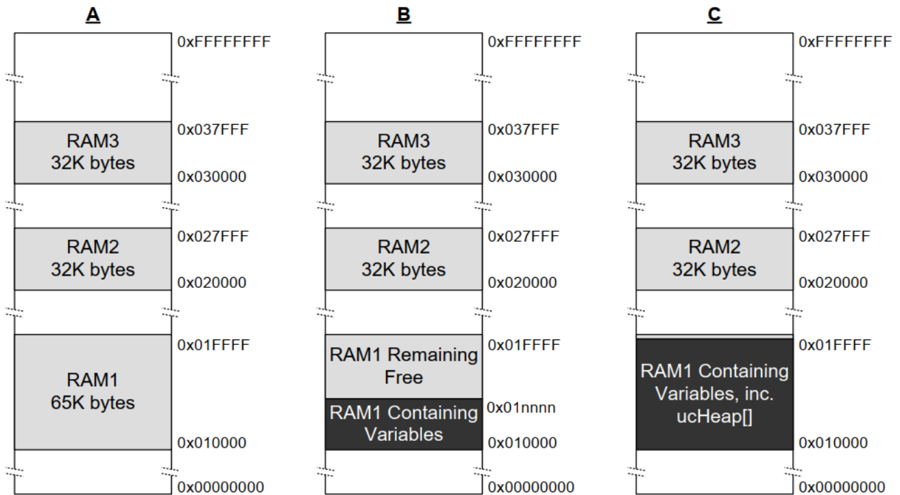
Figure 3.4 Memory Map
