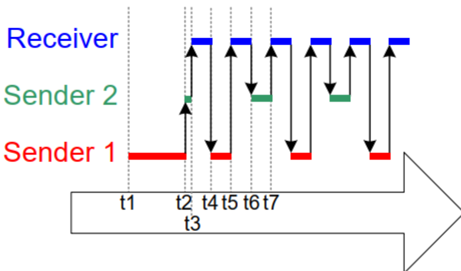
execution produced by Example 5.2
