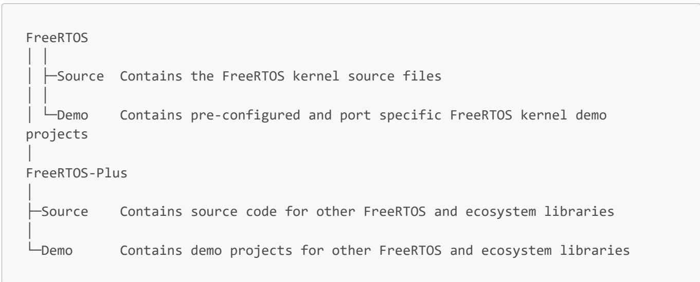
Figure 2.1 Top level directories within the FreeRTOS distribution
